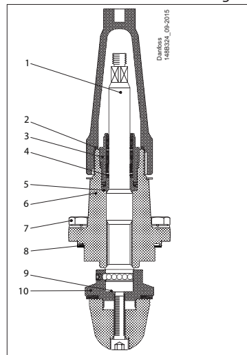
REG-SB 50 / REG-SB 65 manual regulating valve module
