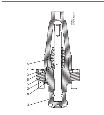
ICF 20 shut-off valve module
