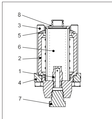
ICFE 20 solenoid valve module
